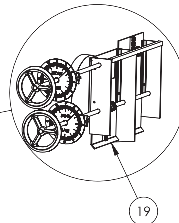
METERING GATE ASSEMBLY (COMPLETE) BAY-LYNX PART# MG100-ASM-1
